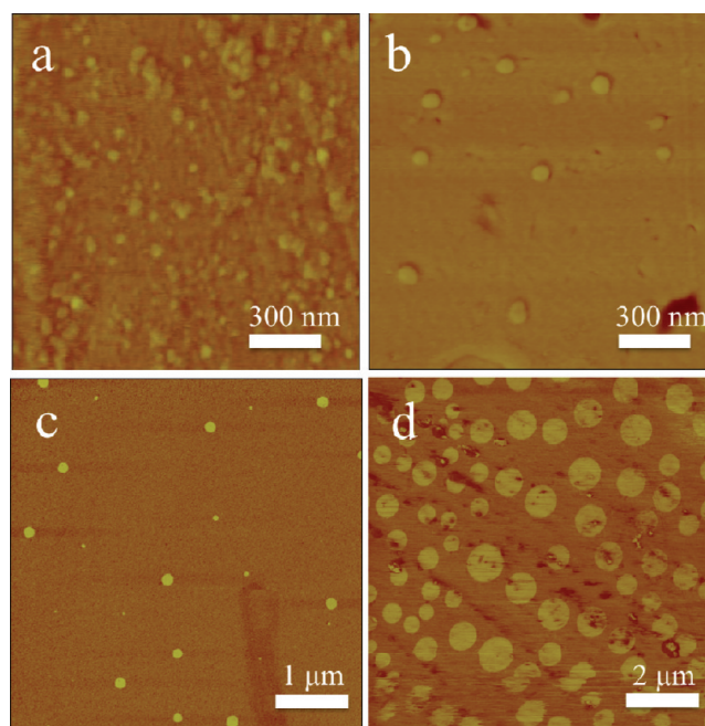
Figure 6. Tapping mode AFM phase images of PS composites loaded with (a) MPS-capped CeO 2 particles, (b) PMMA-grafted CeO 2 particles having a PMMA thickness of 9 nm, (c) PMMA-grafted CeO 2 particles having a PMMA thickness of 29 nm, and (d) PS-PMMA blend without CeO 2 nanoparticles.
