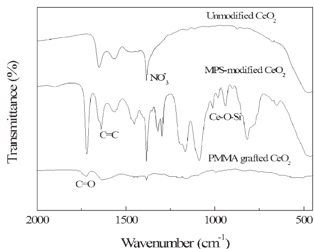
Figure 5. FTIR spectra of unmodified, MPS-modified, and PMMA-grafted CeO 2 particles.
