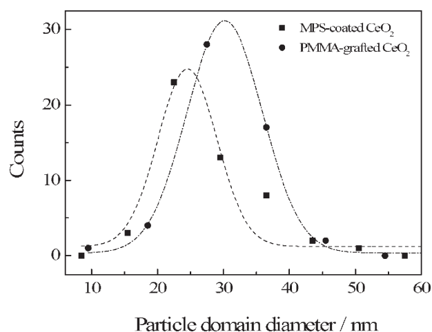
Figure 9. Diameter distributions of MPS-capped \text{CeO}_2 particles (a) and PMMA-grafted \text{CeO}_2 particle domains with PMMA shell thickness of 9 nm. (b) in PS matrix.
