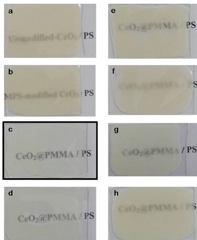
Figure 10. Photographic image of the nanocomposites film prepared by casting. The thickness of the films was around 350 \mu\text{m} . PS composites prepared by (a) unmodified \text{CeO}_2 particles (b) MPS modified \text{CeO}_2 particles, and PMMA-grafted \text{CeO}_2 particles of different PMMA thickness ( t ). (c) t = 9 \text{ nm} , (d) t = 11 \text{ nm} , (e) t = 16 \text{ nm} , (f) t = 29 \text{ nm} , (g) t = 54 \text{ nm} (h) t = 84 \text{ nm} .
