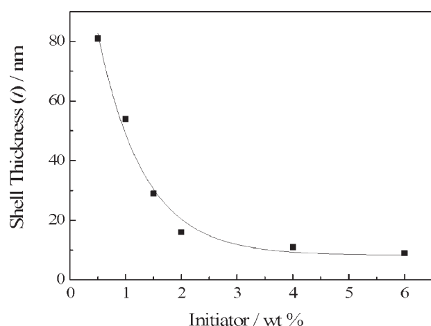
Figure 2. Thickness of PMMA shell on CeO 2 core particle as a function of initiator (BPO) content.
